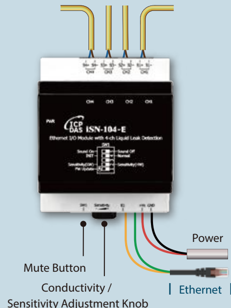
iSN-104-E (4-channel)
