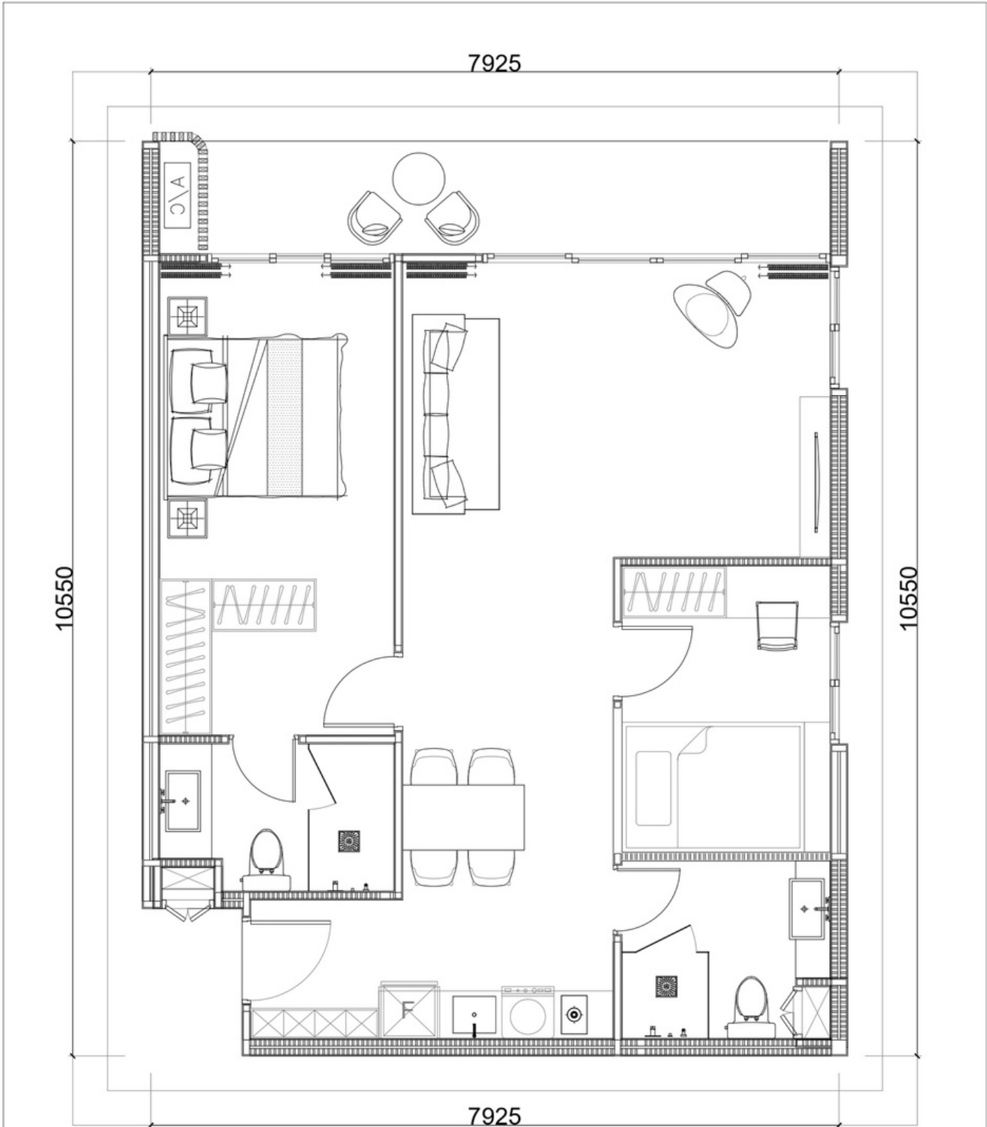
TYPE B/D AREA 78.7 Sq.m
