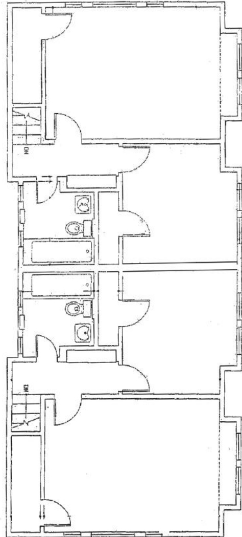
2nd Floor
