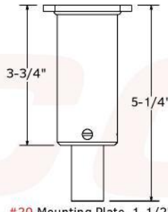
#20 Mounting Plate, 1-1/2" adjustment range, with height adjustable from 3- 3/4" to 5-1/4"
