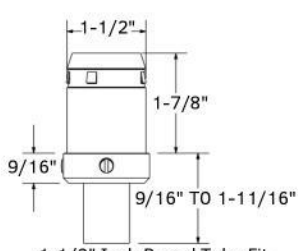
1-1/2" Inch Round Tube Fit Adjustable Range: 1-1/8" Additional Adjustable Height: 9/16" to 1-11/16"
