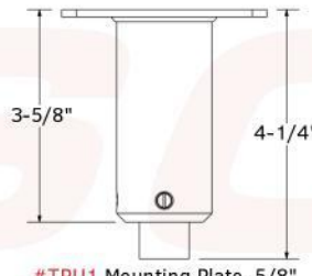
#TPU1 Mounting Plate, 5/8" adjustment range, with height adjustable from 3-5/8" to 4- 1/4"
