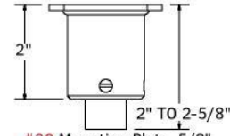
#20 Mounting Plate, 5/8" adjustment range, with height adjustable from 2" to 2-5/8"
