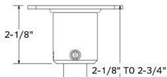
#TPU1 Mounting Plate, 5/8" adjustment range, with height adjustable from 2-1/8" to 2-3/4"
