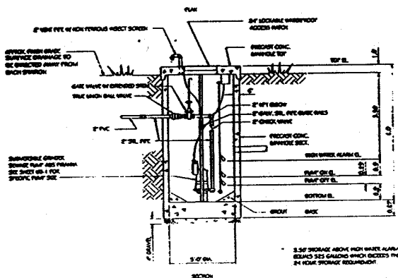
GRINDER PUMP STATION
