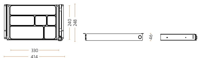
Pen tray - widen model, with removable plastic insert and lock
