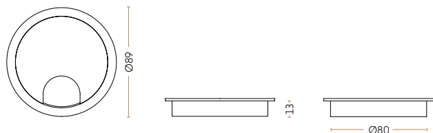
Round cable outlets - \text{\O}80 , and a height on 13 mm.
