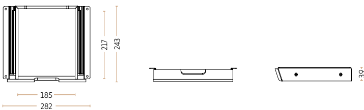
Bamboo Pen Tray x-small 4091-C
