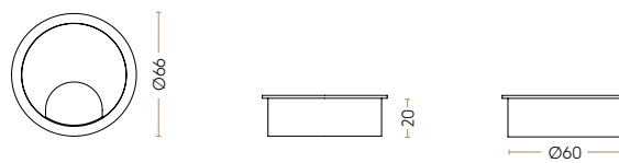
Round cable outlets - \text{\O}60 , and a height on 20 mm.
