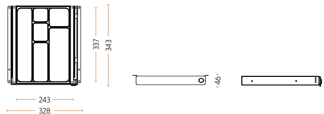
Pen tray - widen model, with removable plastic insert and lock
