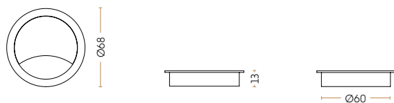
Round cable outlets - \text{\O}60 , and a height on 13 mm.
