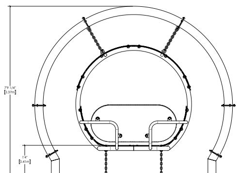
The Suspended FriO | no. H-25004
