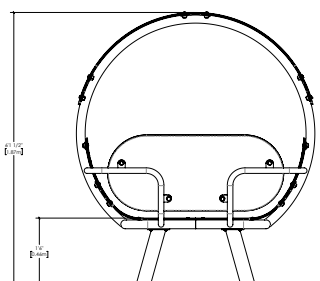
The FriO | no. H-25000 (seat at 18\"/>
