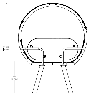
The FriO | no. H-25002 (seat at 30\"/>
