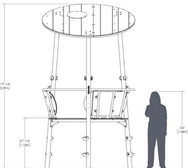
The PlatO | no. H-25006
