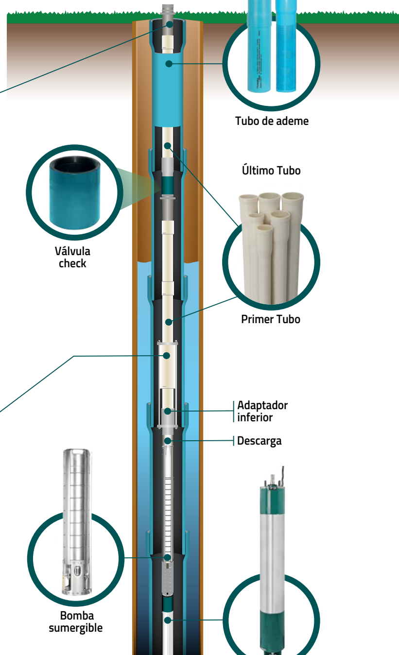
Motor sumergible
