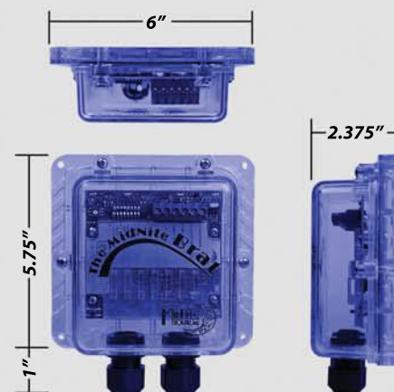
Dimensional View
