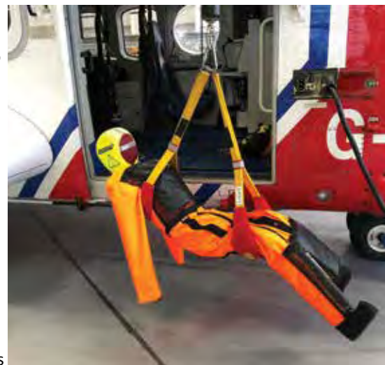
Helicopter Manikin shown with two Single Slings.
