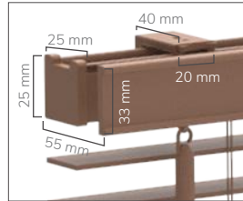
Head Rail
