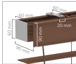
Head Rail
