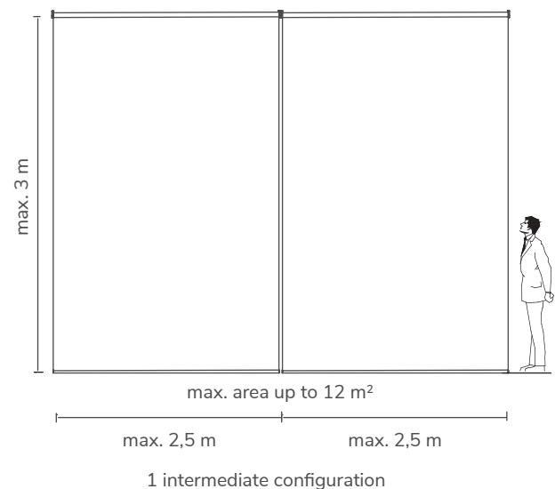
Intermediate System 180°
