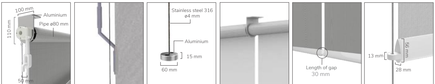
Head Rail
