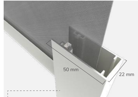
Guide rail section
