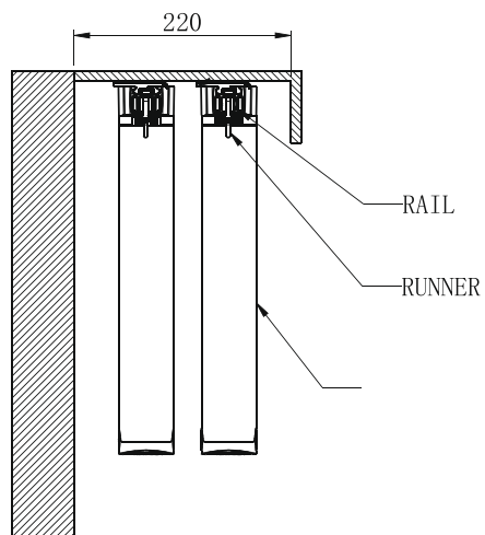
Double Track
