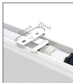
Bracket
