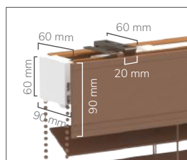
Head Rail
