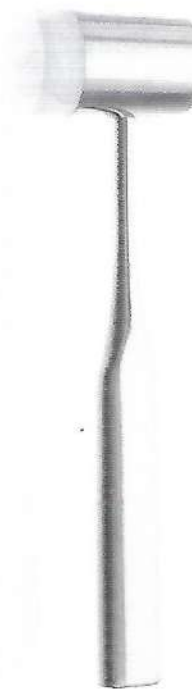
Combination Mallet F9-041 19.5cm 7 5/8" Solid, Head diameter 32.0mm, Weight 12 oz 340 grams, Head weight: 8 oz 227 grams
