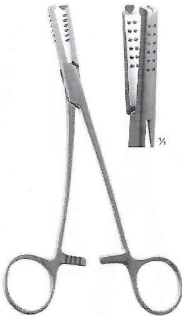
Meniscus Clamp F9-838 18cm 7 1/8" Straight, Curved shaft
