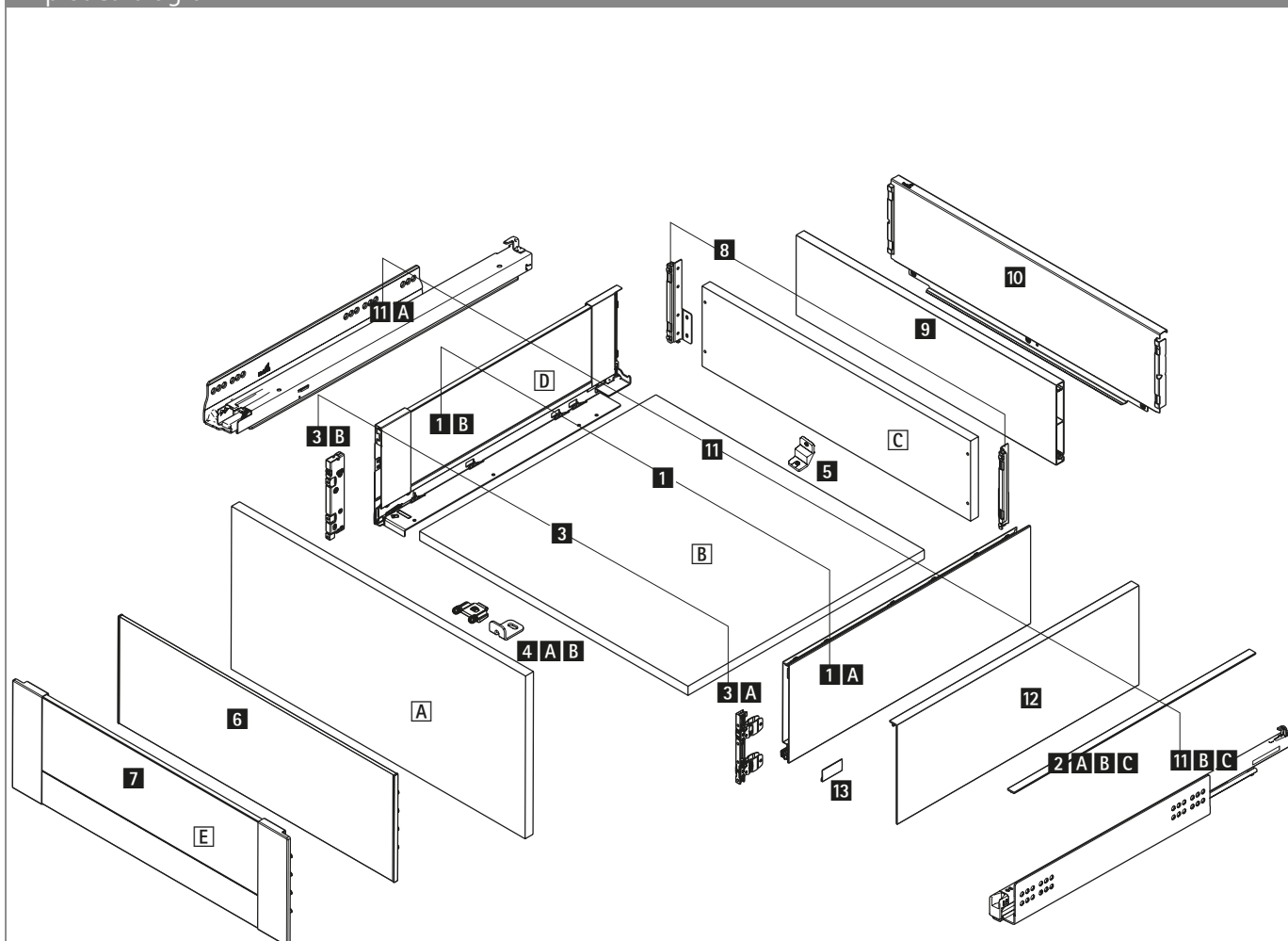
Exploded diagram
