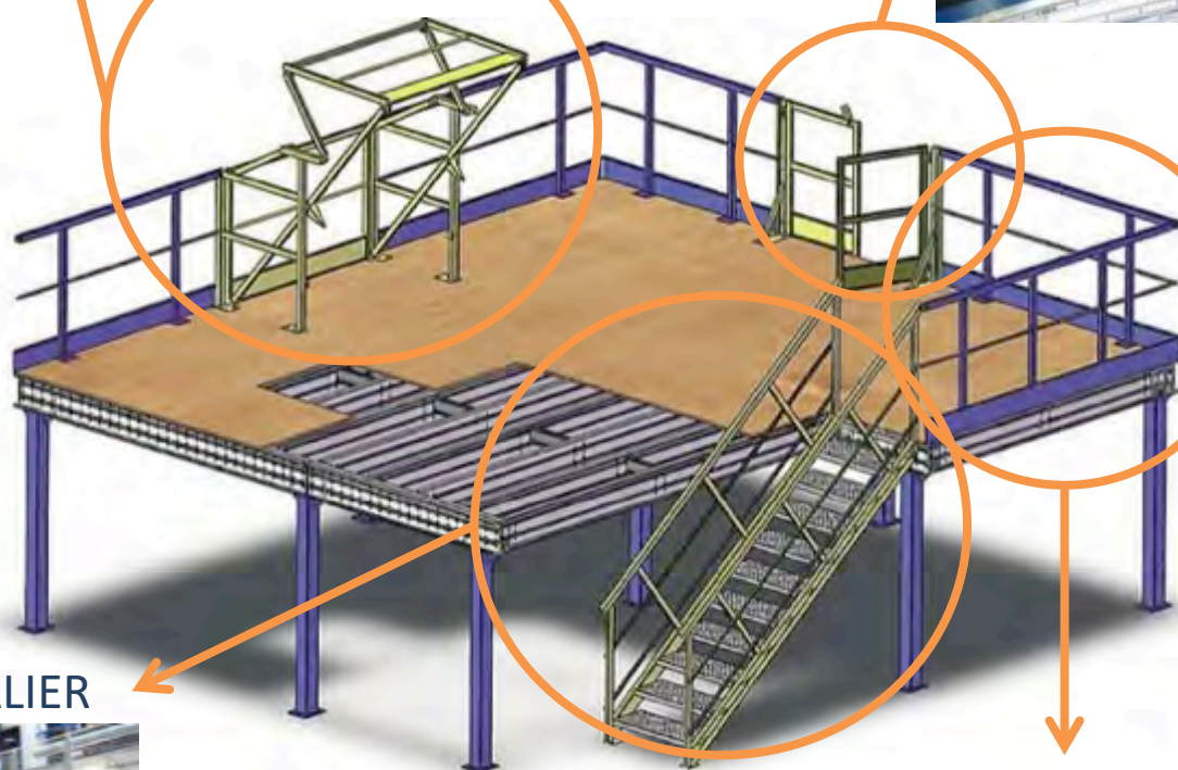
GARDE-CORPS
