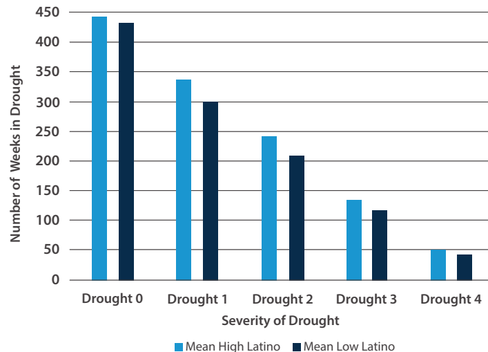
NUMBER OF WEEKS IN DROUGHT: COLORADO 2010-2021
