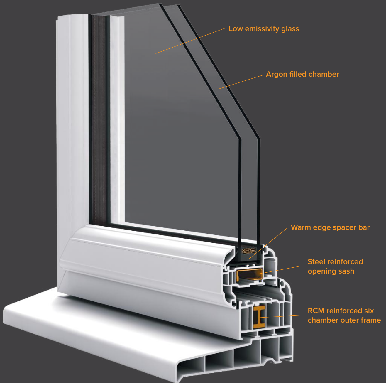
Lorimer casement window cross section
