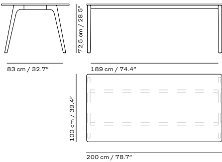
KS432
