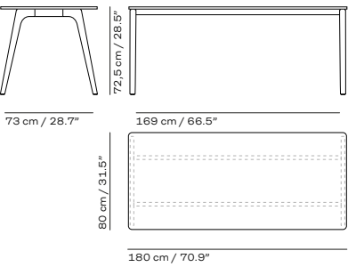
KS431
