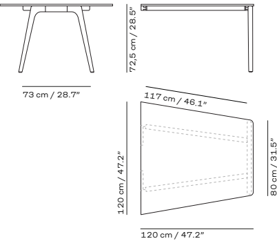
KS437
