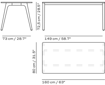
KS430
