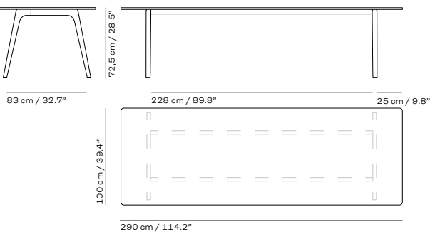
KS434A
