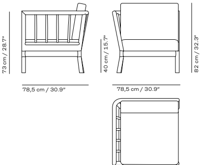
ENDMODUL
