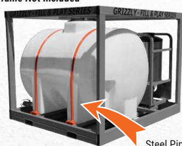
Steel Pipe Straps
