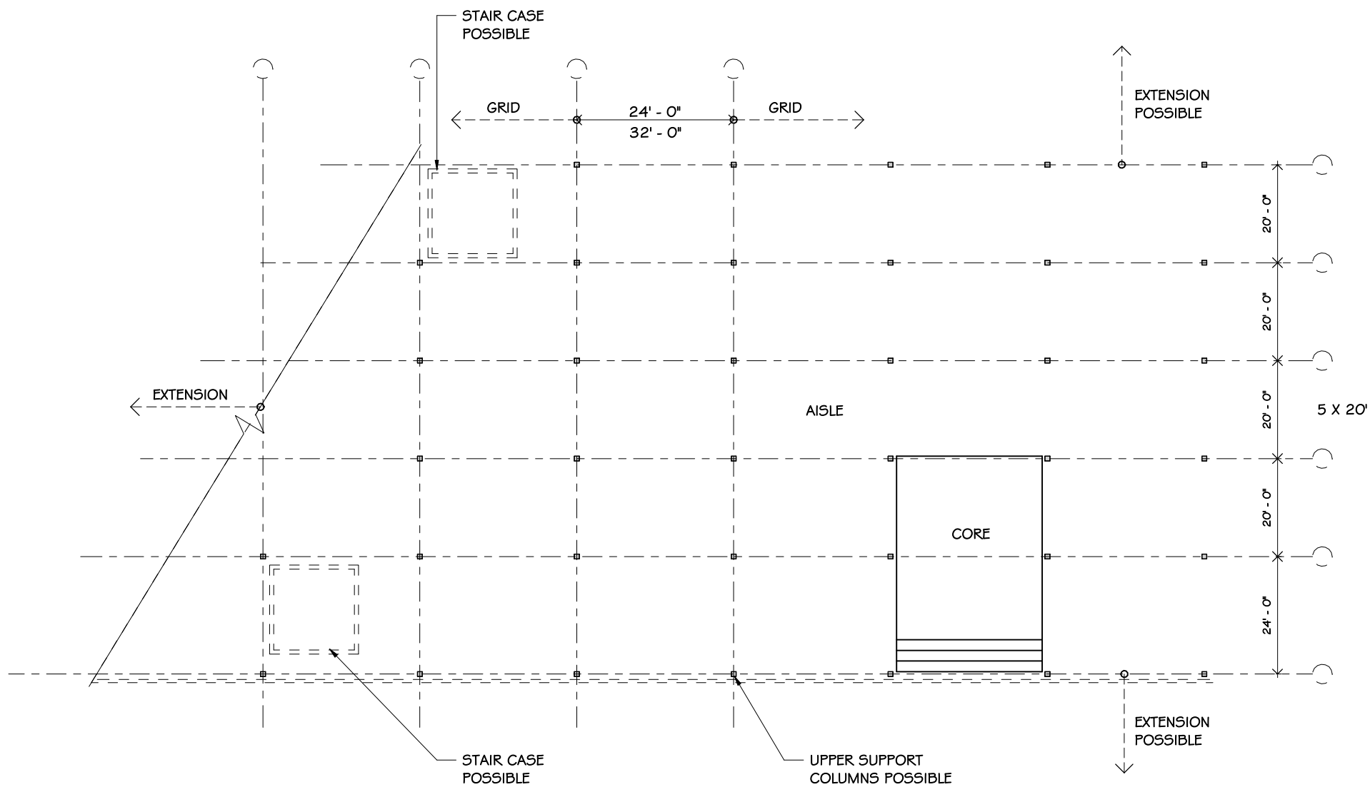
TYPICAL LEVEL
