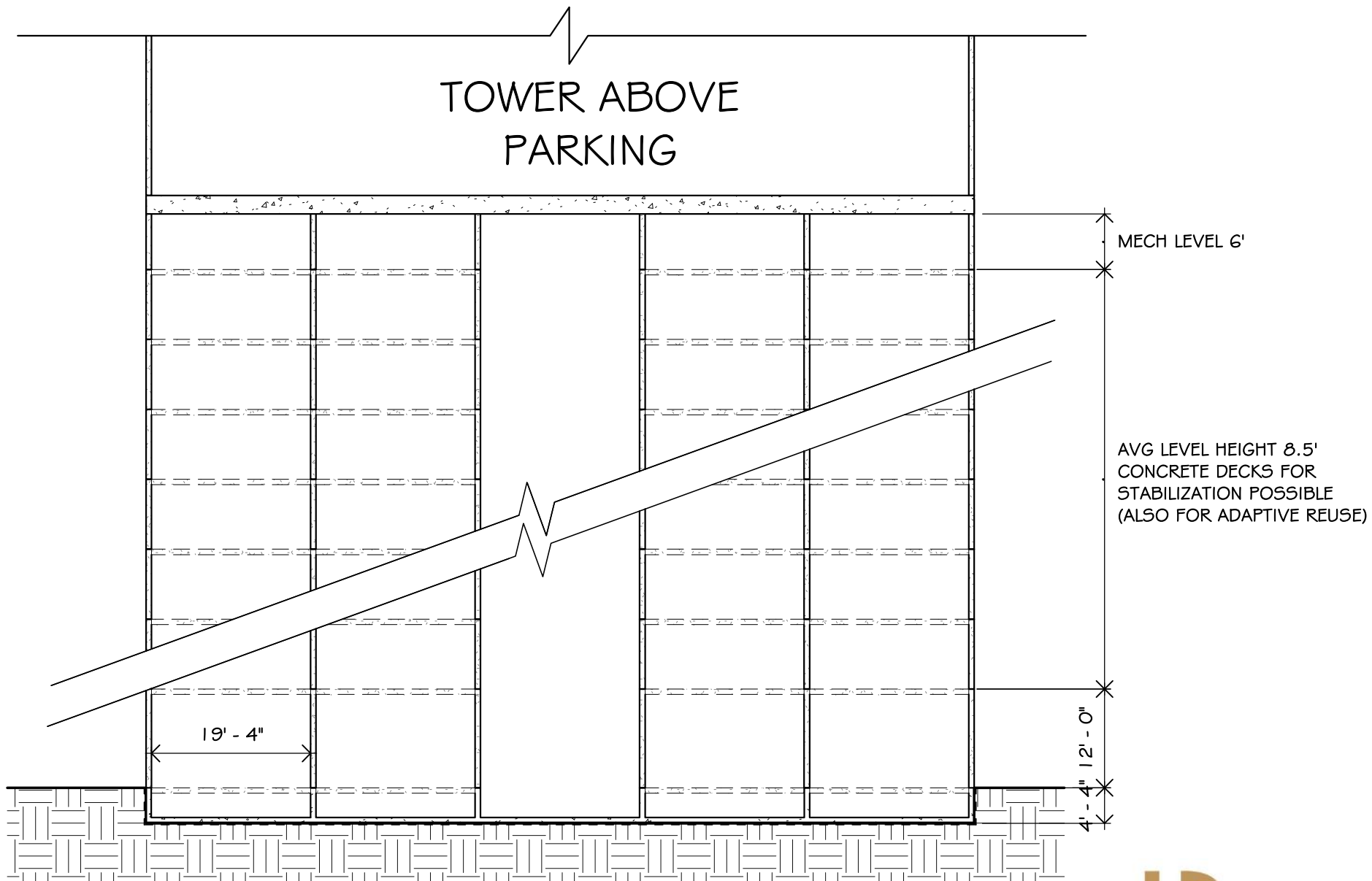
BUILDING SECTION
