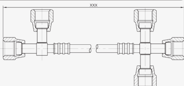
1/4" "T" females at 90° + Cross with 3 1/4" females
