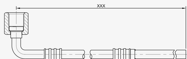
Elbow Female 1/4 + Copper brazing tube
