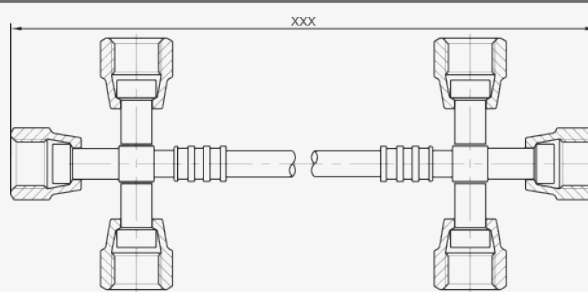
Cross with 3 1/4" females + Cross with 3 1/4" females
