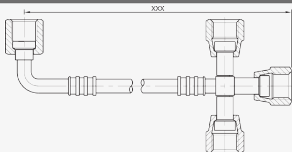
1/4" Elbow Female 90° + cross with 3 1/4" females
