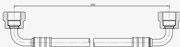
Elbow Female 90° 3/8 + Elbow Female 90° 3/8
