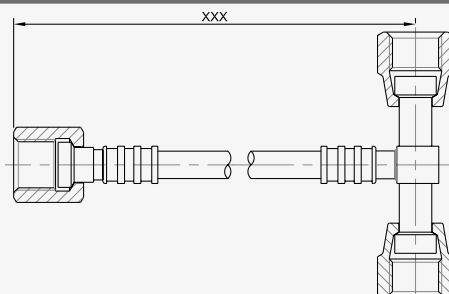
Straight Female 1/4 + "T" with 2 Females 1/4 at 180°
