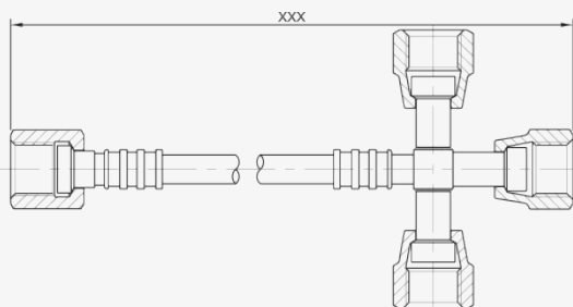
1/4" Straight female + Cross with 3 females
