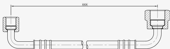
Elbow Female 90° 1/4 + Elbow Female 90° 3/8
