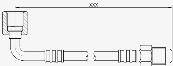
Elbow Female 1/4 + Male 1/4
