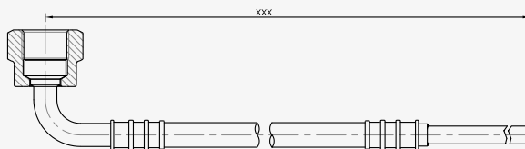
Elbow Female 90° 3/8 + Copper Brazing Tube
