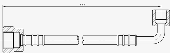
Elbow Female 1/4 + Straight Female 90° 3/8
