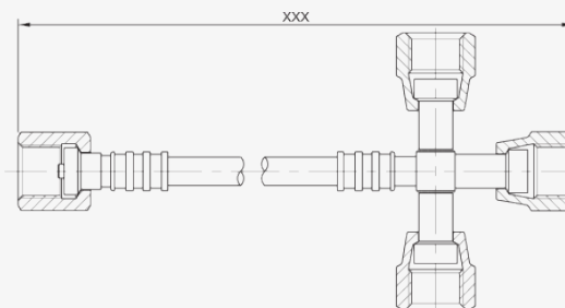
1/4" Straight female with valve opener + cross with 3 1/4" Female
