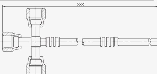
Cross with 3 1/4" females + copper brazing tube
