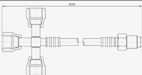
Cross with 3 1/4" females + 1/4" Male
