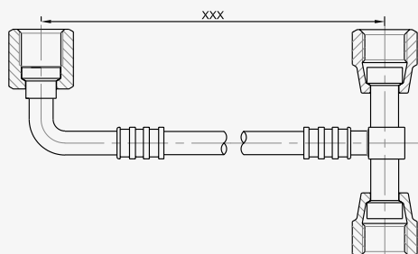
Elbow Female 1/4 + T With 2 Females 1/4 at 180°
