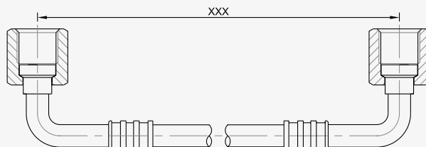
1/4 Elbow Female + 1/4 Elbow Female
