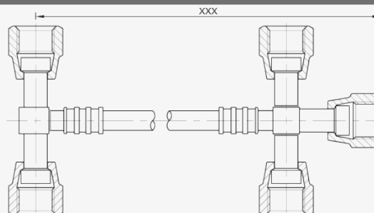
1/4" "T" with 2 females at 180° + 1/4" 3 Females cross
