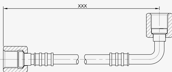
1/4 Straight Female + 1/4 Elbow Female
