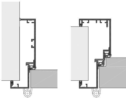
USBV48-E-5-42S Eckzarge, Türblatt 42mm stumpf
