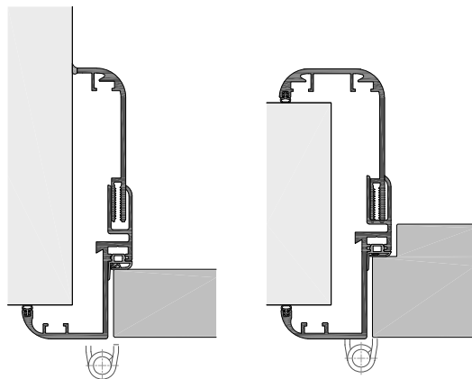
URS48-E-5-42S Eckzarge, Türblatt 42mm stumpf
