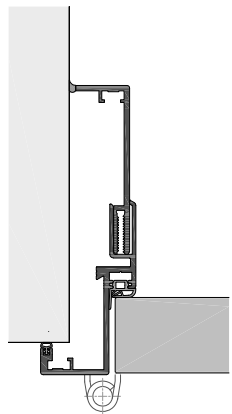
UST48-E-5-42S Eckzarge, Türblatt 42mm stumpf
