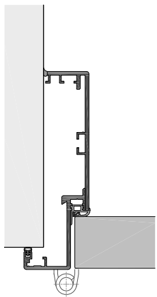
USTB48-E-5-42S Eckzarge, Türblatt 42mm
