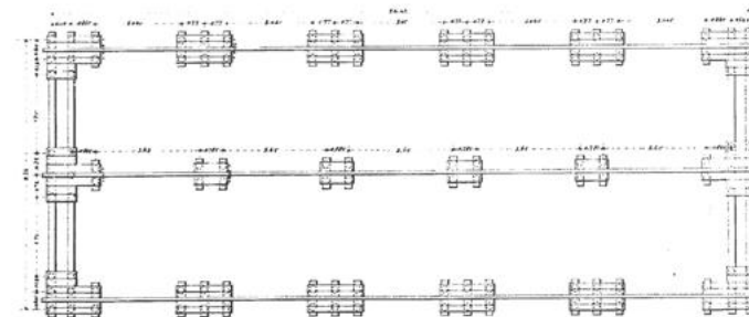
PAALFUNDEERING.
