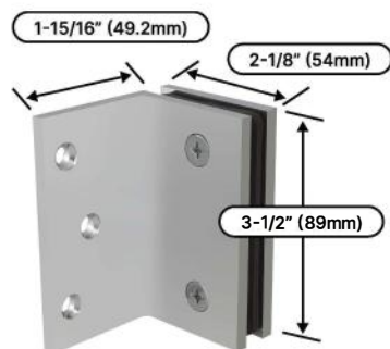
WMB90 Square Wall Mount Bracket - 90°
