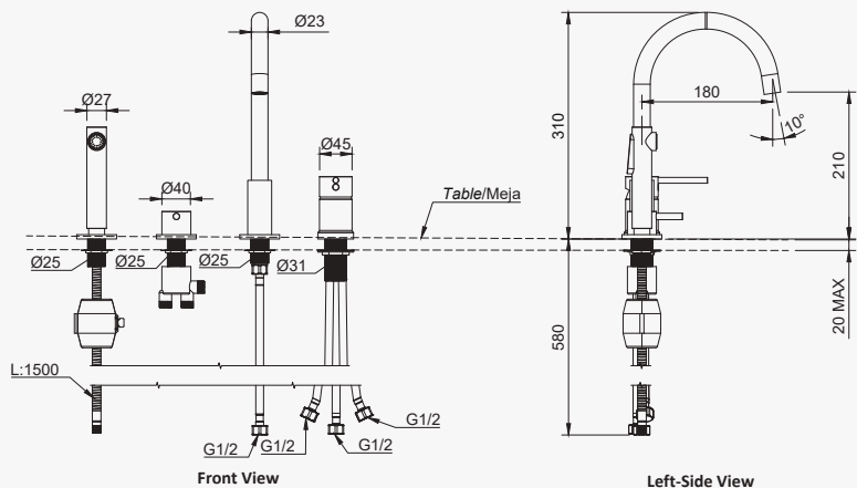
AT215BGM Banyan 4 Hole Kitchen Mixer with Spray Brushed Gunmetal
