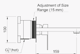
Left-Side View
