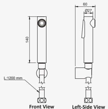
AT313BBC Banyan Jet Shower Brushed Copper
