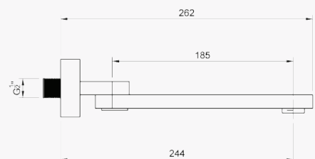
Left-Side View
