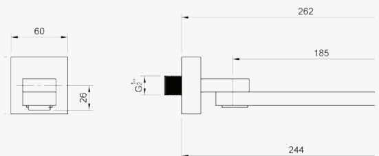
Left-Side View
