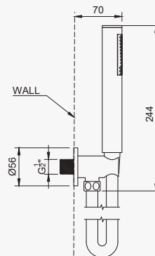
Left-Side View
