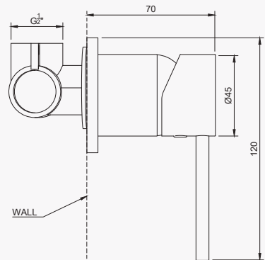
Left-Side View
