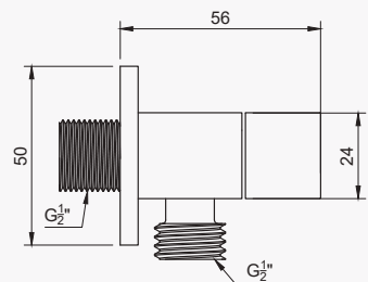
Left-Side View
