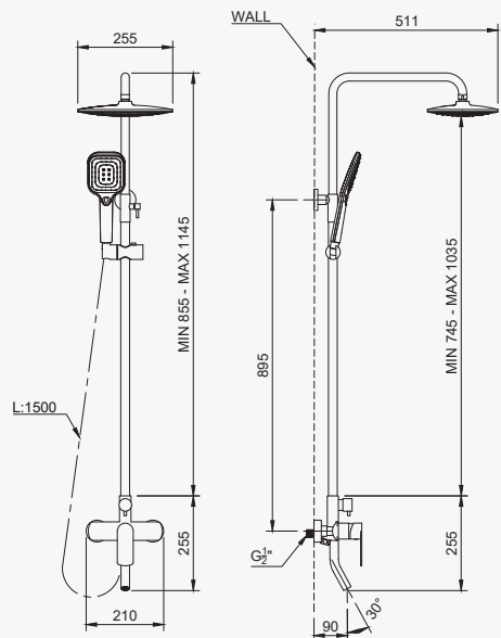
Left-Side View
