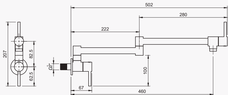
Left-Side View
