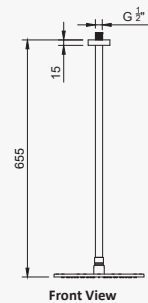
AT122BBCC60 Banyan Ceiling Mounted Fix Head Shower H:600mm Brushed Copper
