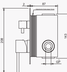
Left-Side View
