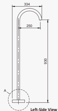
Left-Side View
