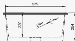
Left-Side View
