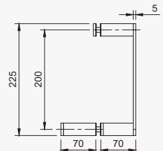
Left-Side View
