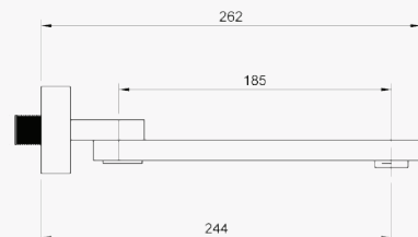
Left-Side View
