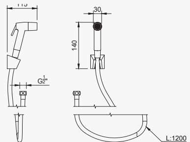
Left-Side View
