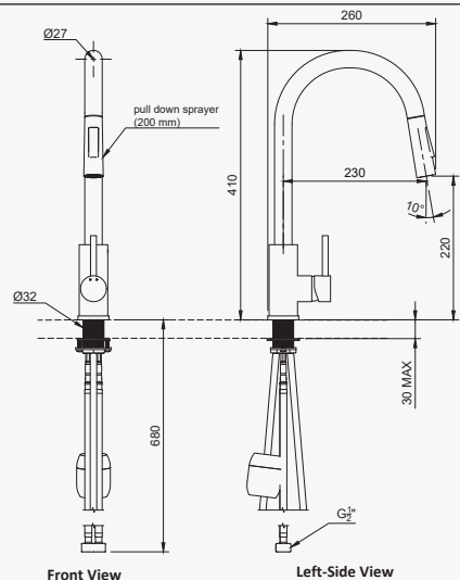
AT213BBC Banyan Extendable Hose Kitchen Mixer Brushed Copper
