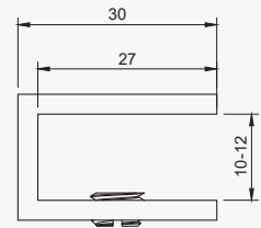
Left-Side View
