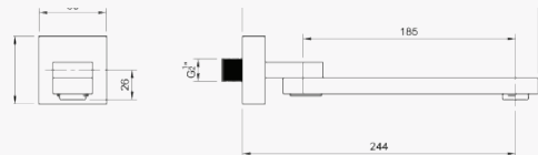
Left-Side View
