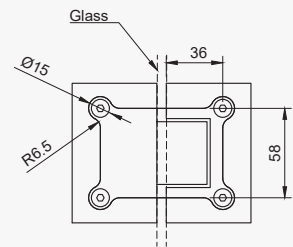
Detail View
