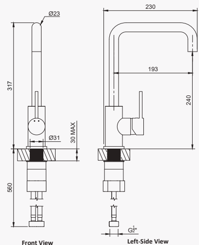
AT213B2BC Banyan V2 Kitchen Mixer Brushed Copper
