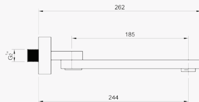
Left-Side View
