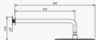
Left-Side View
