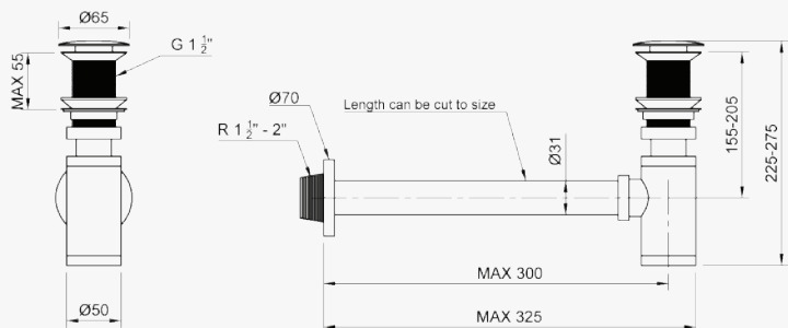
Left-Side View
