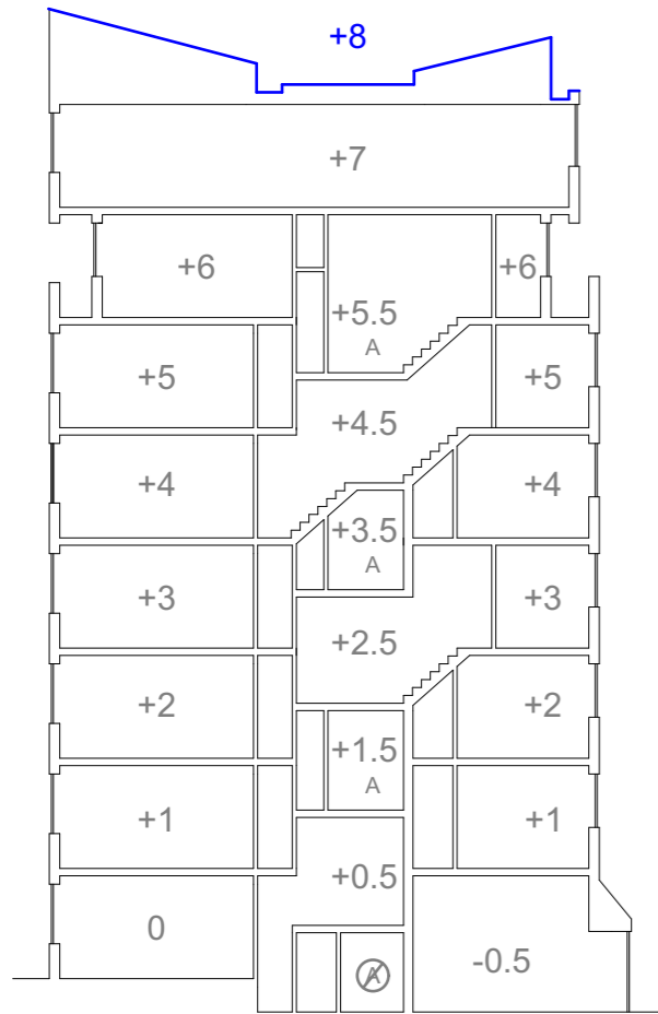
CROSS SECTION
