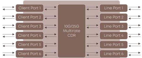
Functional scheme
