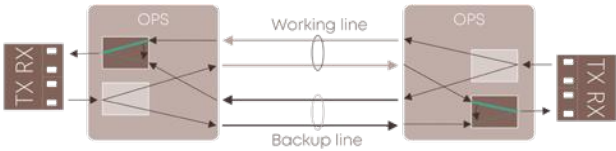
Functional scheme
