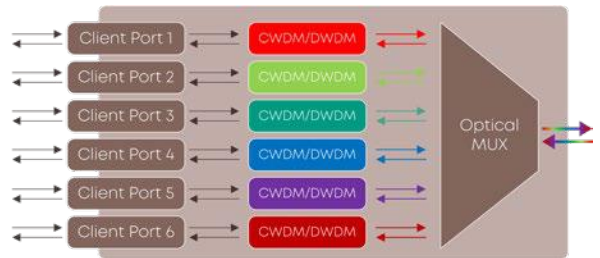
Functional scheme
