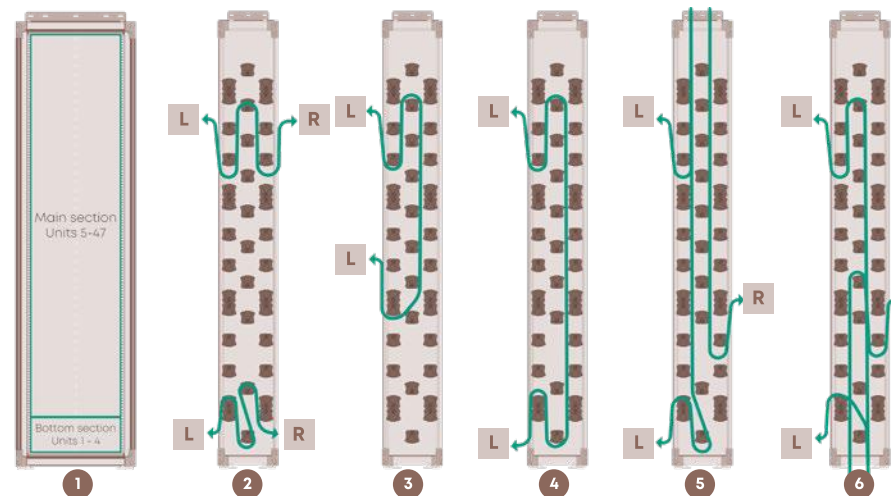
Patching lengths
