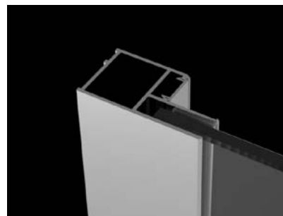
Torrenta, Eos – Profile + 2 cm (except from Eos I, Torrenta PDJ). You should replace standard U profile with the extension profile P01-284195001.
