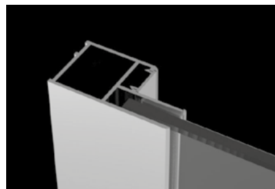
Idea – profile + 2 cm. You should replace standard profile with the extension profile on the side of the fixed wall P01-ID-KDJ-SC-01.
