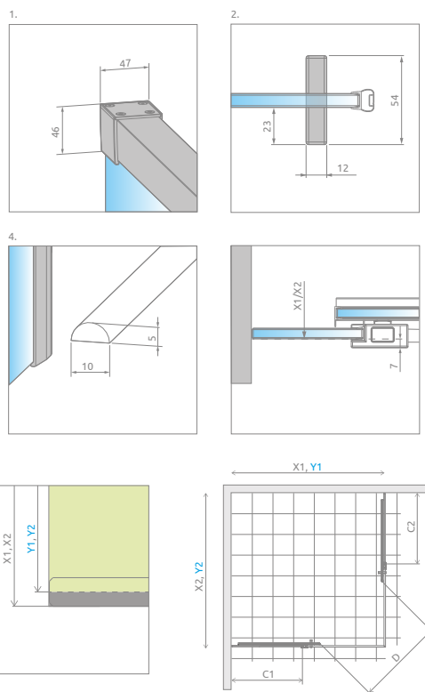
XL Size – installation without a shower tray
