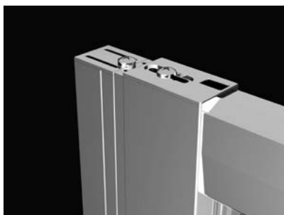
Premium Pro – profiles +2 cm. You should add the extension profile to the standard U profile on the side of the fixed wall. P01-293199801.
