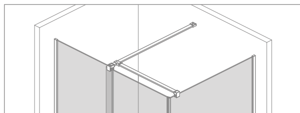
Perpendicular cross stabilizer
