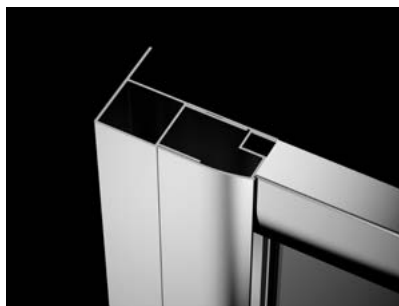
Vesta – profile +2cm. You should replace standard U profile with the extension profile P01-120150001.
