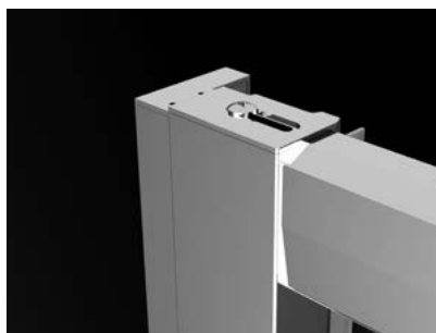
Premium Pro – standard U profile on the door side.
