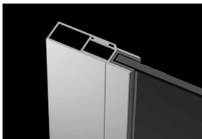
Carena – Profile + 2 cm. You should replace standard U profile with the extension profile P01-133195001.
