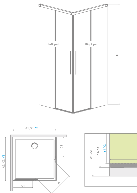
Standard size – installation on the shower tray
