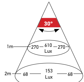
EuroLED 130
