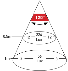
5000 K - 12 LED
