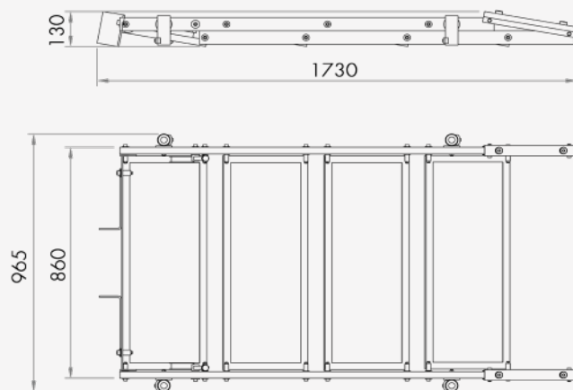
FOLDED DIMENSIONS
