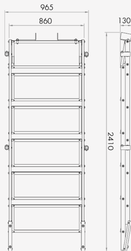
FOLDED DIMENSIONS
