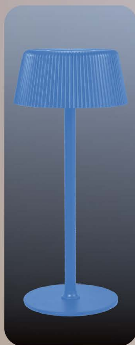
TL6001-AZUL. LED 3W. Dimerizable. USB-C. 3000/4000/6500K Variables. Ø11,5×26,5cm. Azul.
