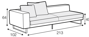
3 seater left / or right back cushion 54x54 and 72x54
