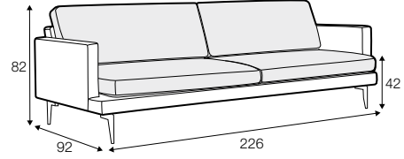
3 seater with 2 cushions
