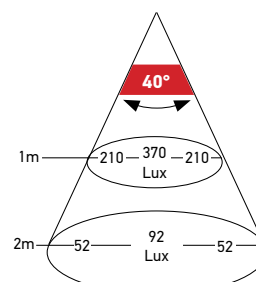
EuroLED 150
