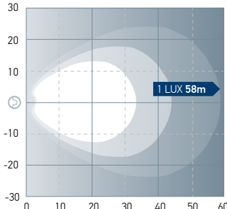
Module 70-S Close Range 2.5m high at -10°
