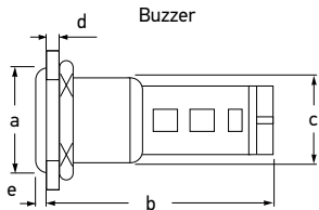
Buzzer
