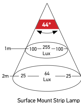
Surface Mount Strip Lamp
