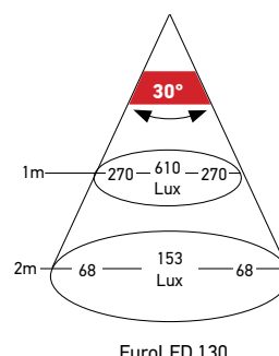
EuroLED 130 Shroud Black 9HD 959 027-002 White 9HD 959 027-012
