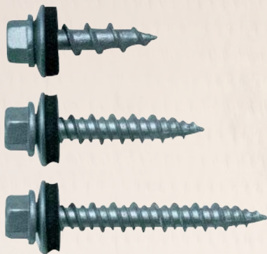
Hex Washer Head, AF 1/4", #8 Washer, Metal to Wood Screw, Type 17 Cutter
