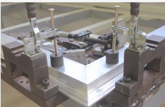
Jig Fixtures
