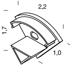
BP23ENDCAPS End caps
