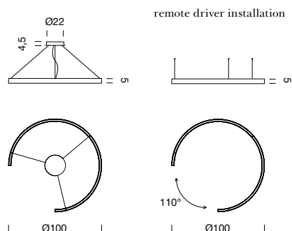
remote driver installation
