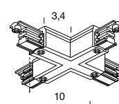
X-FEED
