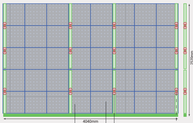
Front/Back view
