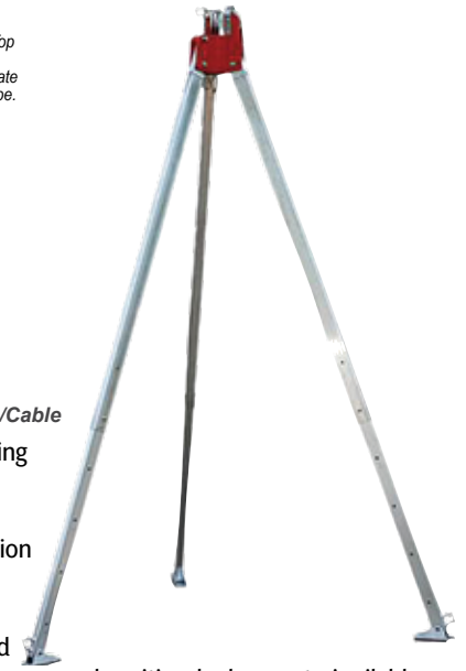
Swivel Eye Rigging Points (2) Spring-Lock Mechanism Locks Legs into Place
