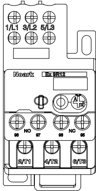
AD51 shown with Ex9R12 for reference only
