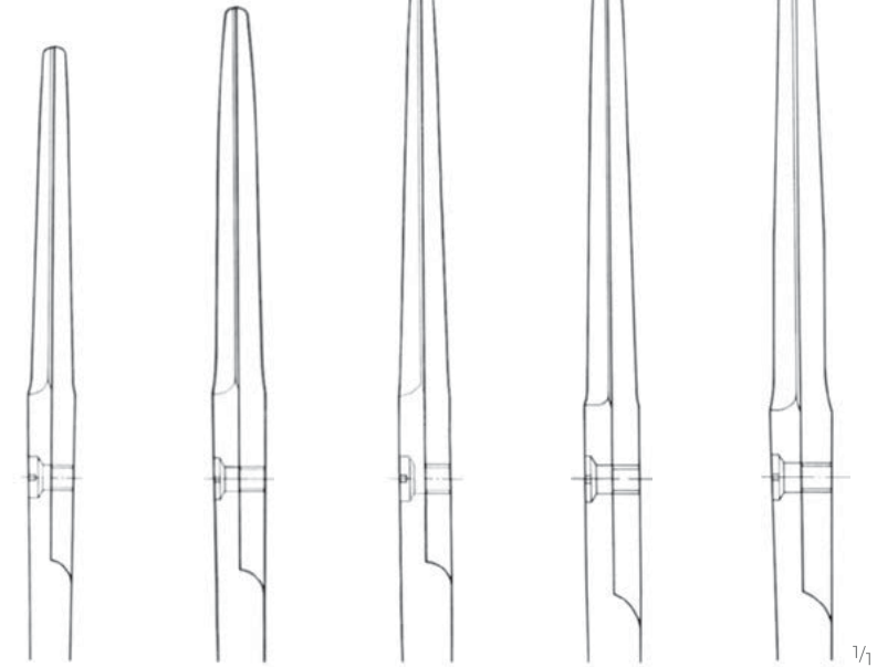
MC 01.101.239 13.5 cm MC 01.101.240 14.5 cm MC 01.101.241 15 cm MC 01.101.242 16.5 cm MC 01.101.243 17.5 cm
