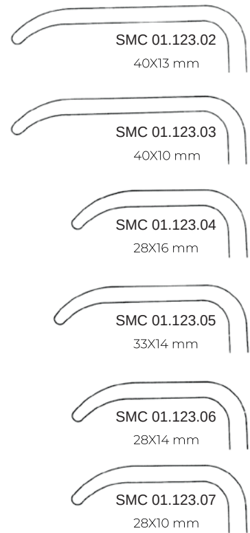
LANGENBECK SMC 01.123.07-SMC 01.123.02 21 cm
