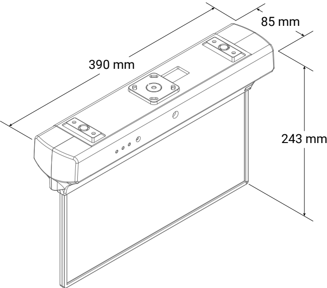
ORTHOGRAPHIC DRAWING
