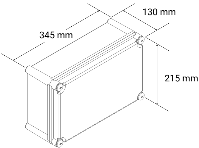
ORTHOGRAPHIC DRAWING
