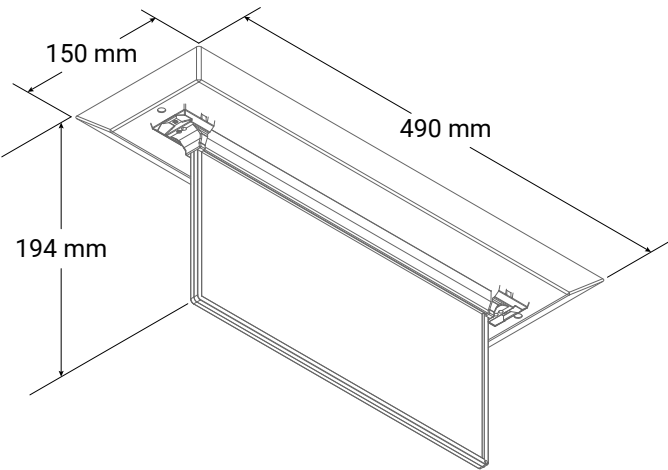
ORTHOGRAPHIC DRAWING
