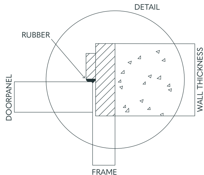
FRAME WITHOUT ARCHITRAVE
