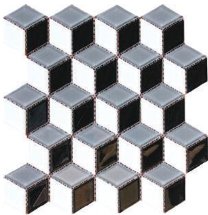
CUBE 1 SHEET SIZE: 270mm x 293mm CHIP SIZE: 65mm x 75mm x 4mm KM334.C1
