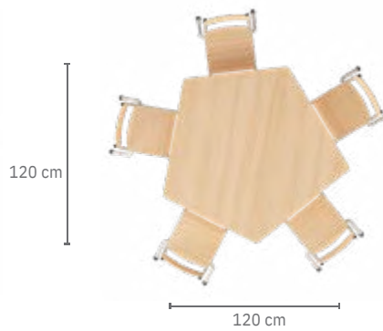
■ Small Pentagon Table 120 x 120 cm
