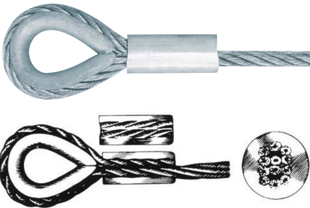
Cross section of a splice showing how rope and ferrule form one strong, homogenous mass.
