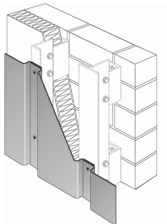
Panel with concealed connection
