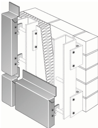
Cassette façades with invisible fixings
