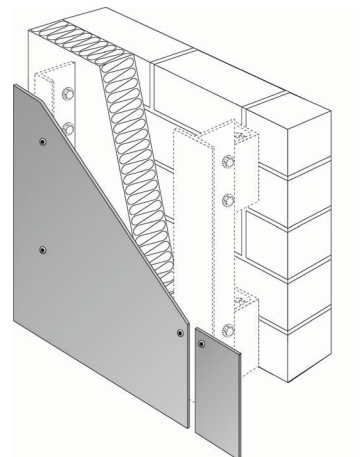
Flat sheet / Riveted
