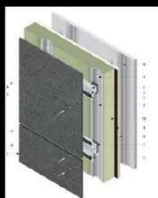
RIVET SYSTEM
