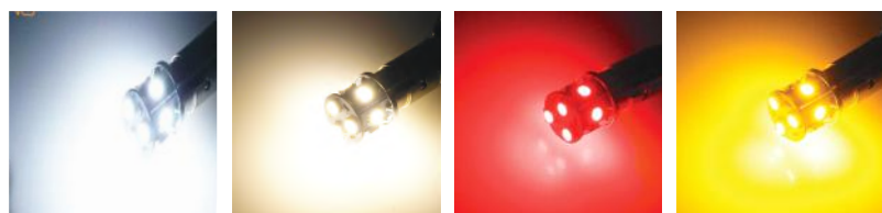
Part No. 4635015XW – Xenon White Part No. 4635015WW – Warm White Part No. 4635015RO – Red Part No. 4635015AG – Yellow BA15S 5W – 9 SMD LED'S Multivolt 10-30V, set of 2pc € 19,95 excl. VAT / € 23,74 incl. VAT
