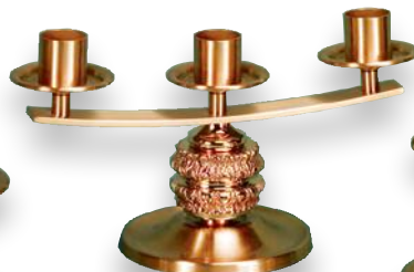
71ACL30 Height 5 1/2", Base Diameter 6 5/8" C $1,100 ea. $1,195 ea. 5 Lite $1,300 ea. $1,465 ea. 7 Lite $1,570 ea. $1,770 ea.
